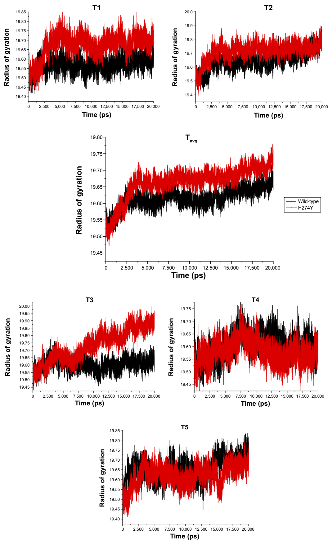
Figure 7 Radius of gyration average comparison across the 20 ns molecular dynamic simulation of WT HINI and H274Y HINI : T1, T2, T3, T4, T5, and T avg presenting the five individual 20 ns molecular dynamic trajectories and overall average, respectively.
